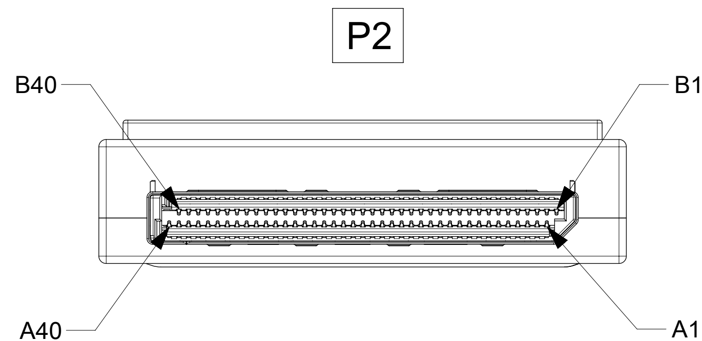
VIEW FROM MATING END OF CONNECTOR
